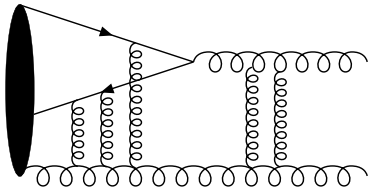
Fig. 1. Non-perturbative interactions of O(1) in the spectator model
